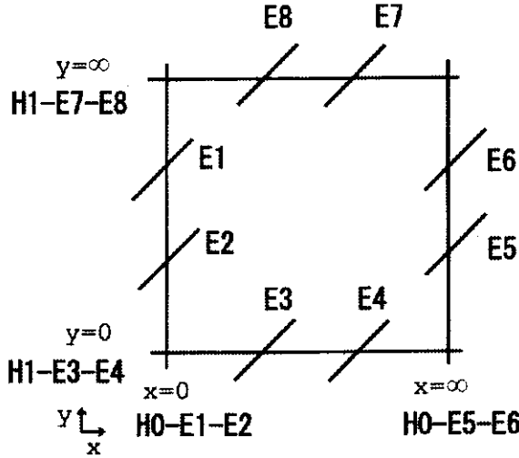
Fig. 1. Irreducible divisors and their intersections
